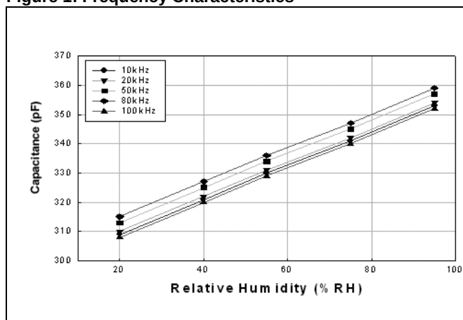
Figure 1: Frequency Characteristics
