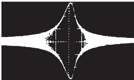
Second order bandpass filter f_o = 100 \text{ kHz} ; Q = 30 ; \text{Gain} = 4
