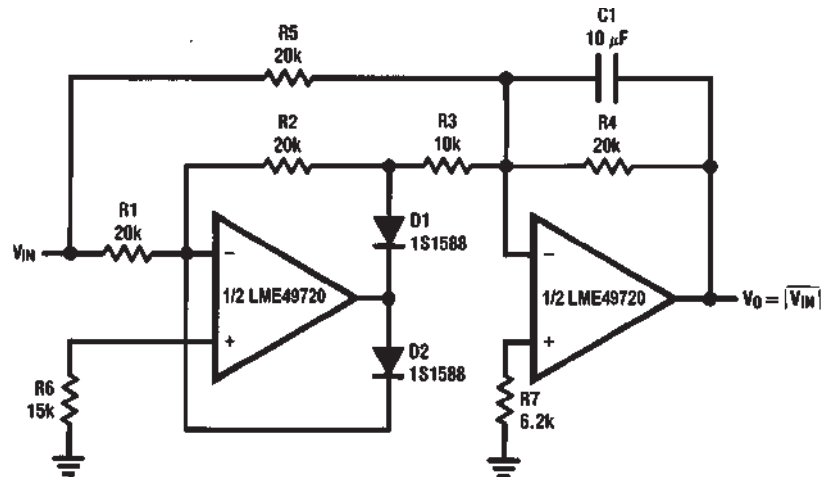
Figure 119. AC/DC Converter
