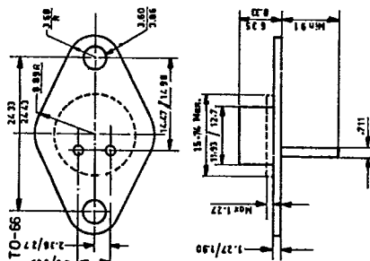
TO-66
