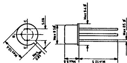
TO-39
