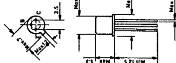
TO-18
