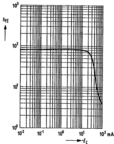
DC current gain h_{FE} = f(I_C) -V_{CE} = 10 \text{ V}; T_{\text{case}} = 25^\circ\text{C}
