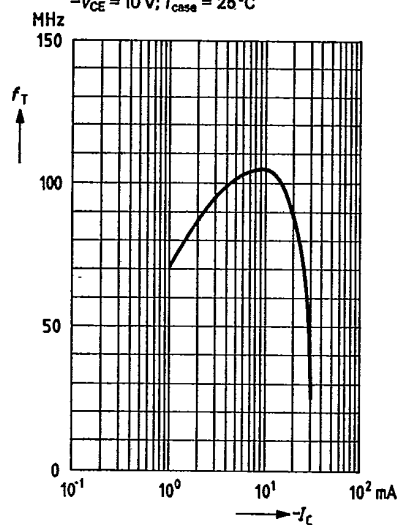
Transition frequency f_T = f(I_C) -V_{CE} = 10 \text{ V}; T_{\text{case}} = 25^\circ\text{C}
