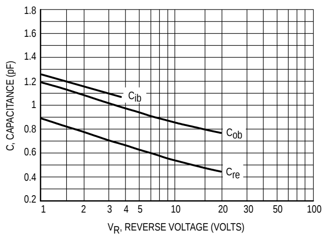
Figure 4. Capacitances
