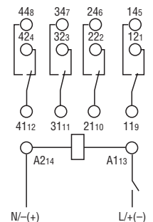
Wiring diagram (without signal START)
