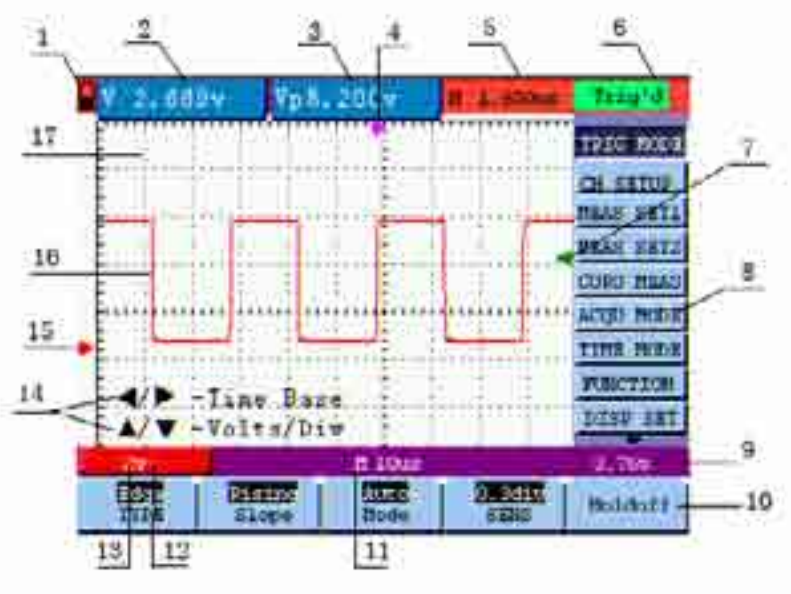
figure 4: Oscilloscope Operation Window
