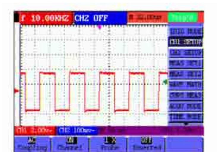
Figure 35: AC Coupling
