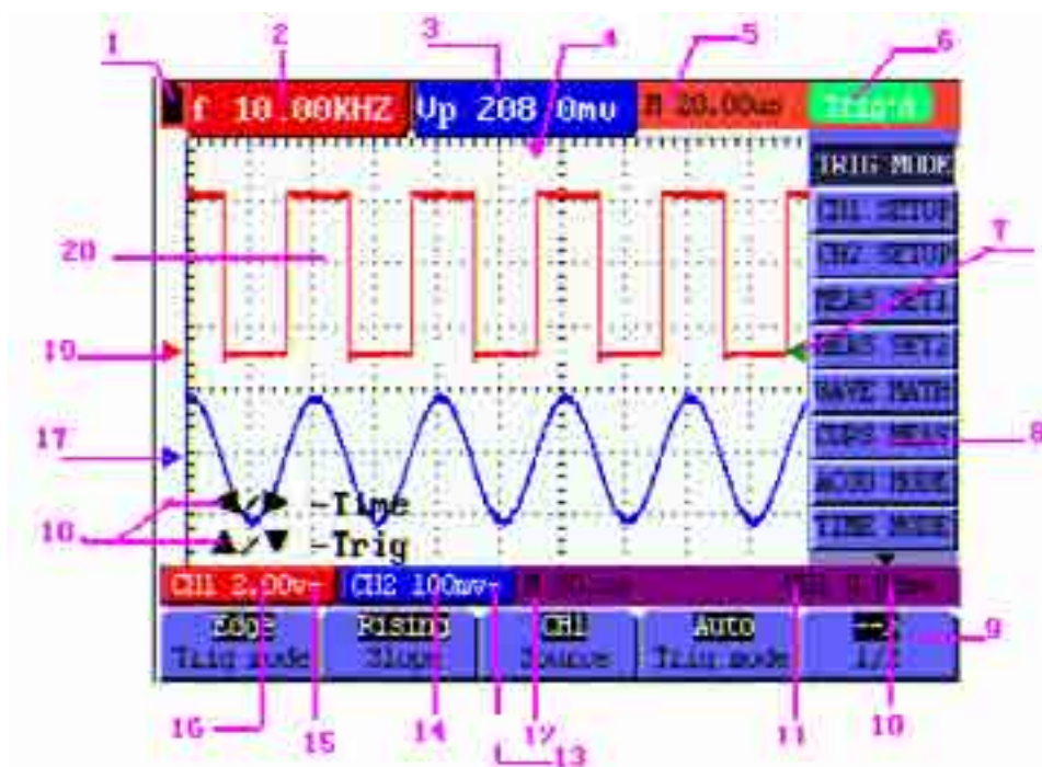
Figure 5: Oscilloscope Operation Window
