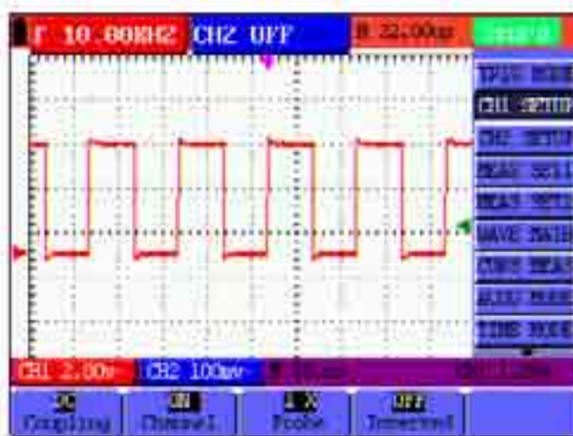
Figure 36: DC Coupling
