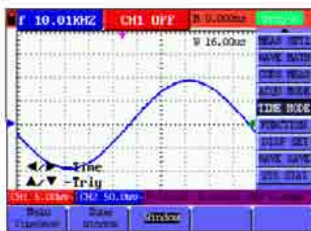
Figure 68: Window Extension
