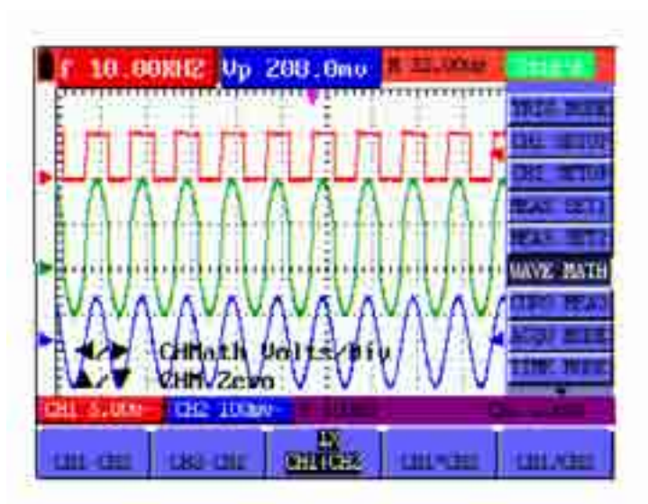
Figure 19: Waveform Mathematics
