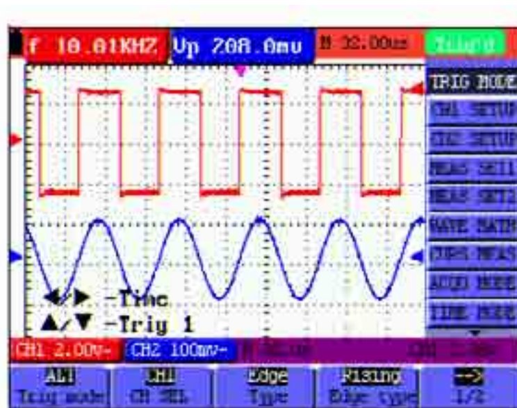
Figure 44 Alternate Trigger
