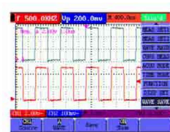
Figure 49: Waveform Saving
