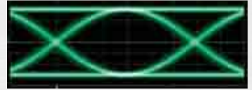
Open eye with 2.5 Gb/s serial data signal. At this data rate, the probed signal is mostly unaffected by serial data channel response.
