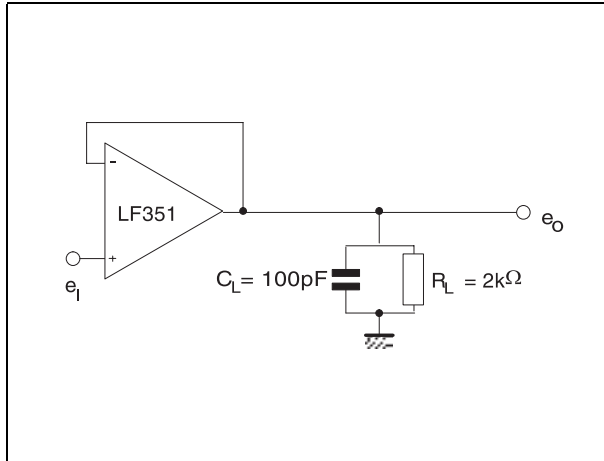
Figure 20. Voltage follower
