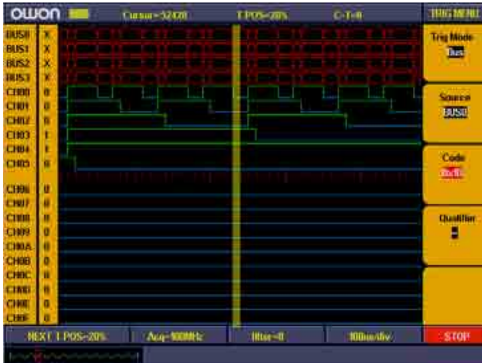
Fig.5-57: Bus trigger
