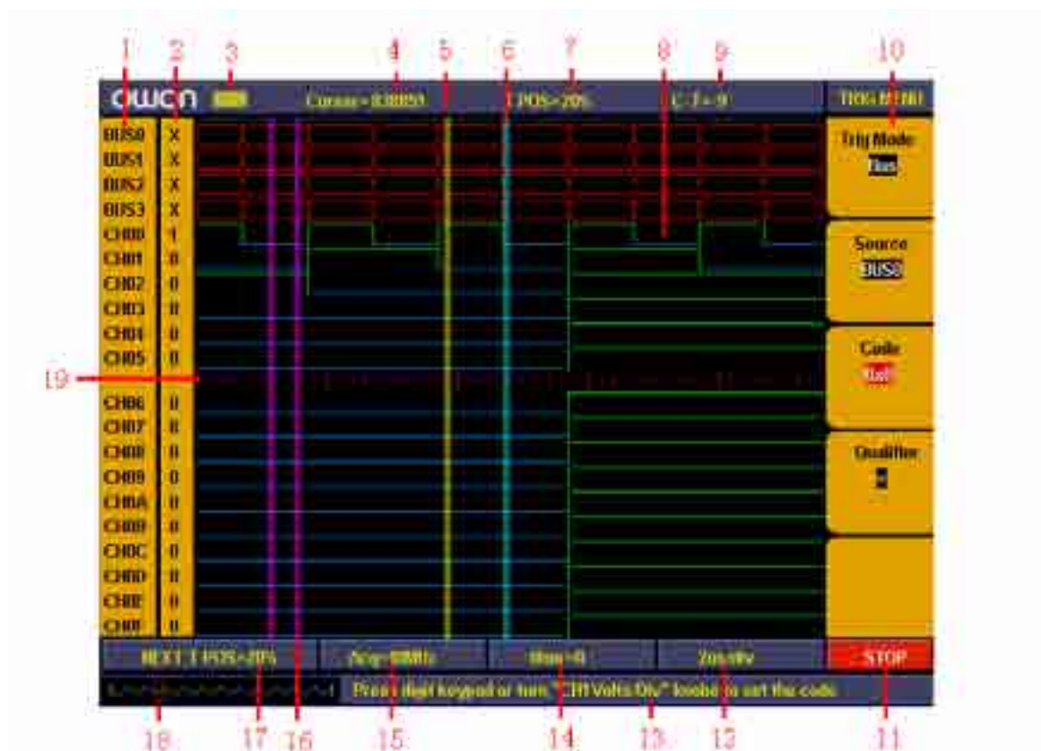
Fig.4-12: User interface of logic analyzer
