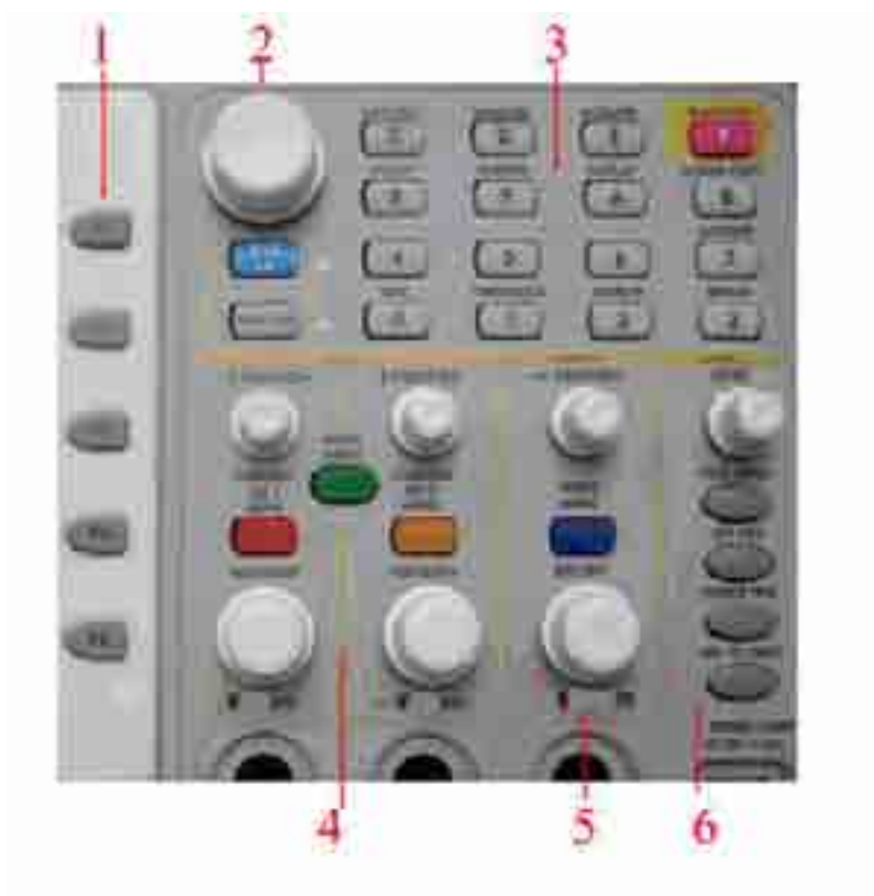
Fig. 4-2 Keys Overview
