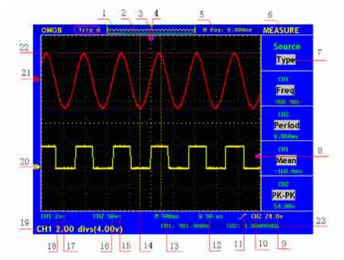
Fig. 4-3 Illustrative Drawing of Display Interfaces
