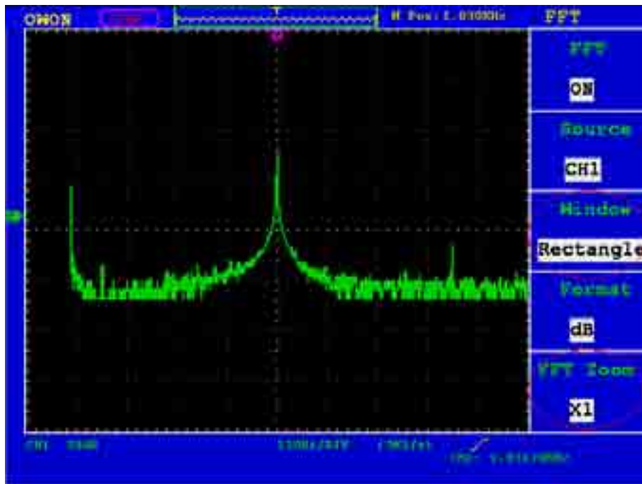
Fig.5-11. Rectangle window
