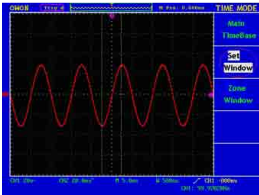
Fig. 5-16 Window Setting
