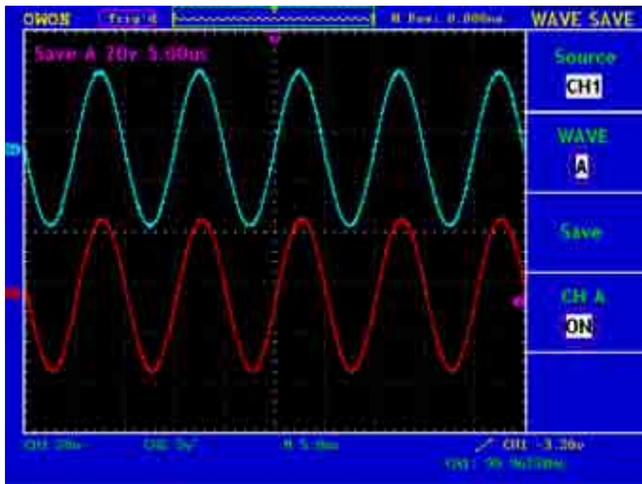
Fig.5-38 Wave Saving
