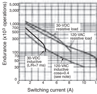
Endurance G5LE
