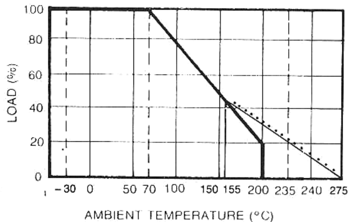
DERATING CURVE
