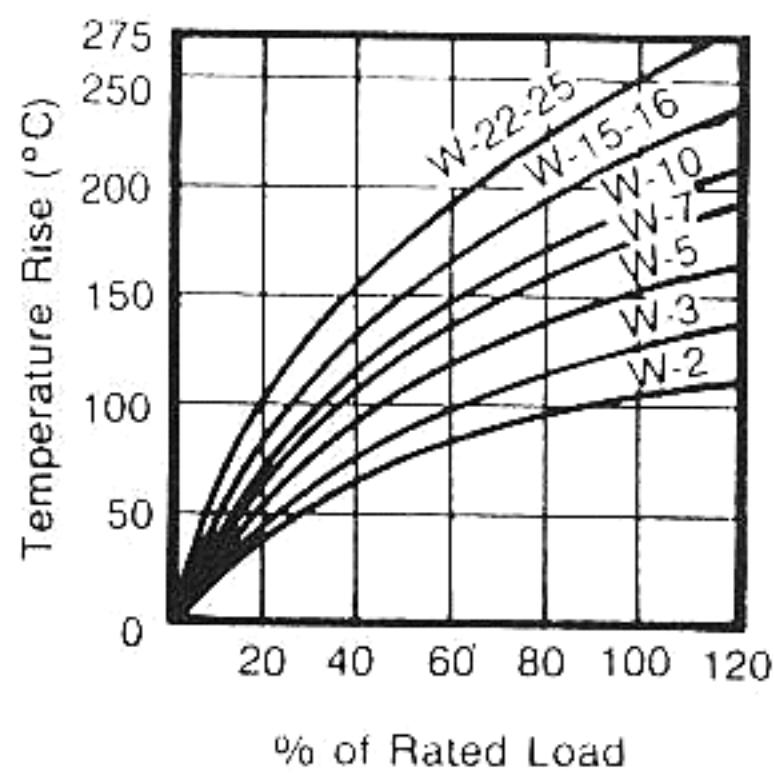
TEMPERATURE RISE AT 25°C
