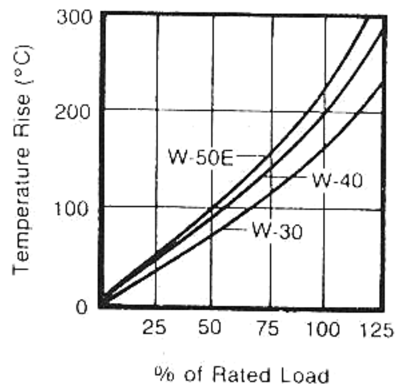
TEMPERATURE RISE AT 25°C (Without Bracket)
