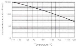
Insulation Resistance VS. Temp.
