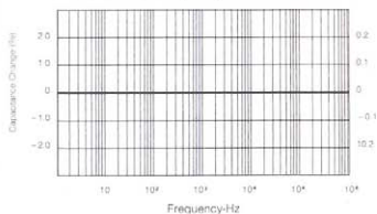
\Delta C , D.E. VS. Frequency Coefficient
